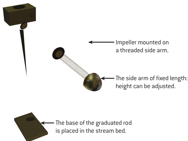
▲ Figure 2.5.7 Impeller
