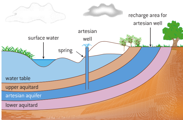
▲ Figure 4.2.2 Aquifer structure
