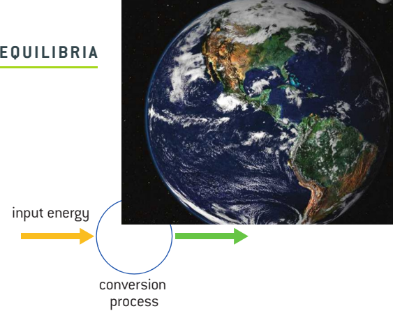
▲ Figure 1.3.3 The second law of thermodynamics
